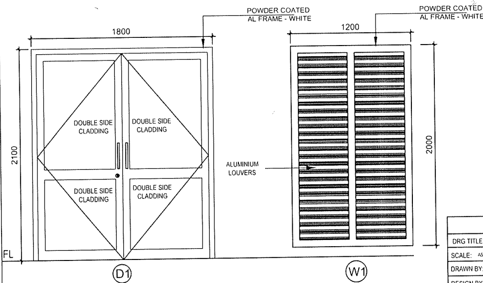
DOOR WINDOW DETAIL
