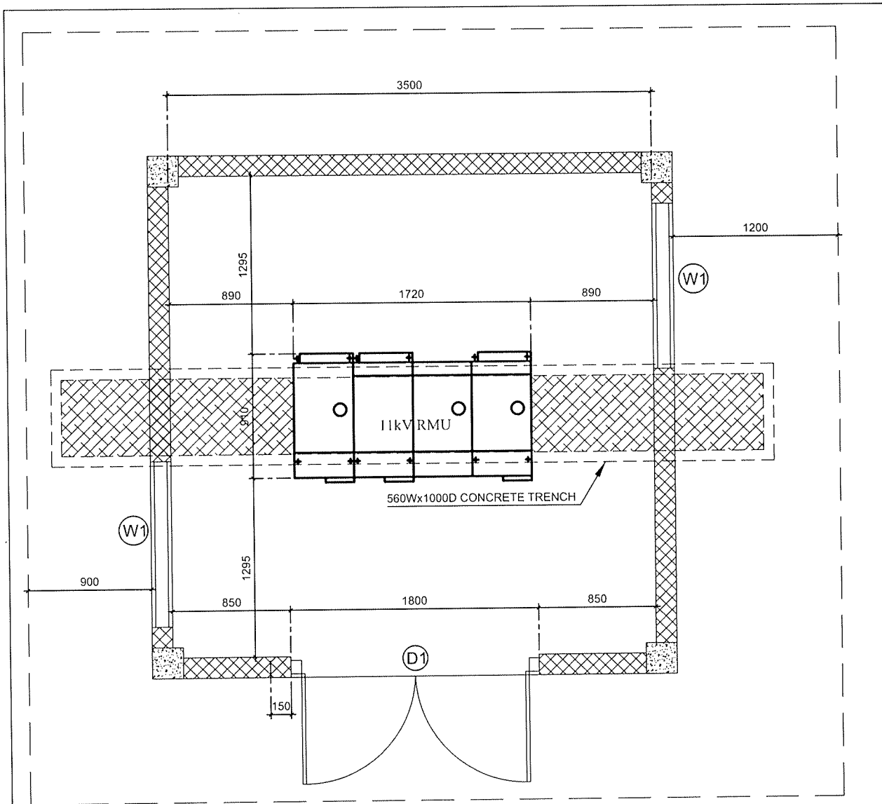
FLOOR PLAN
