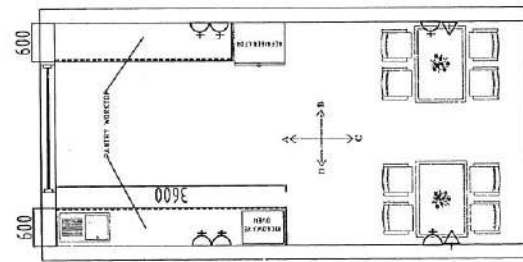
PLAN AT WORK TOP LEVEL
