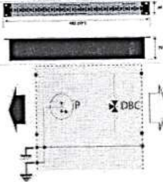
P: 3-electrode GDT DBC Low capacitance diode
