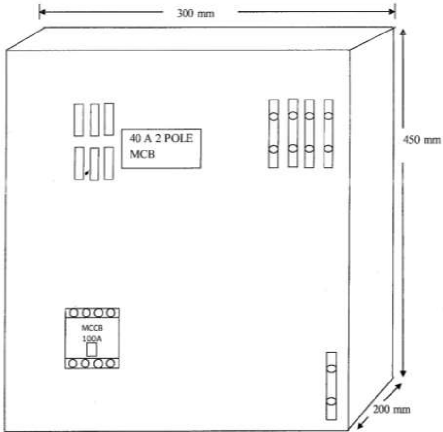
(Inside of cover plate arrangement)
